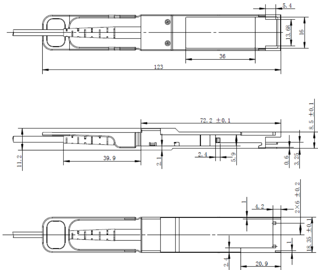
Figure 3. Outline Drawing
